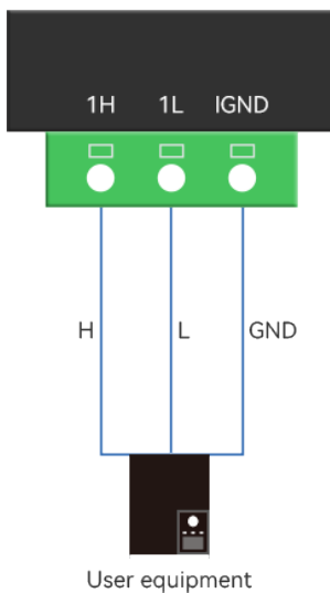
CAN Wiring Diagram
