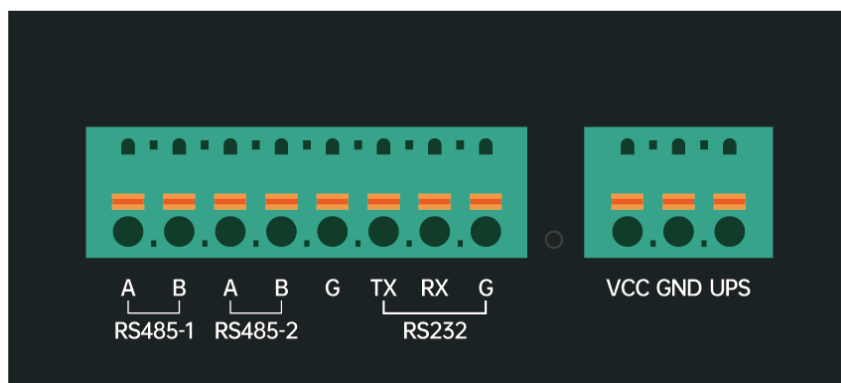
EG8200mini Interface Identification-2
