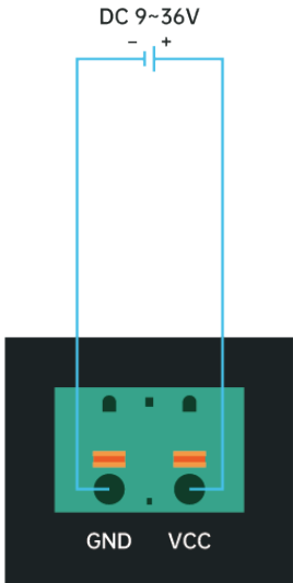
Power Wiring Diagram
