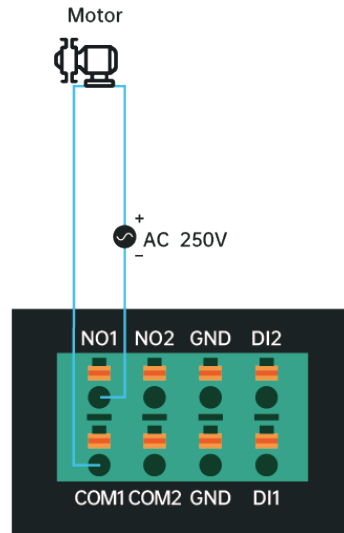
DO Wiring Diagram
