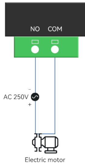
DO Wiring Diagram
