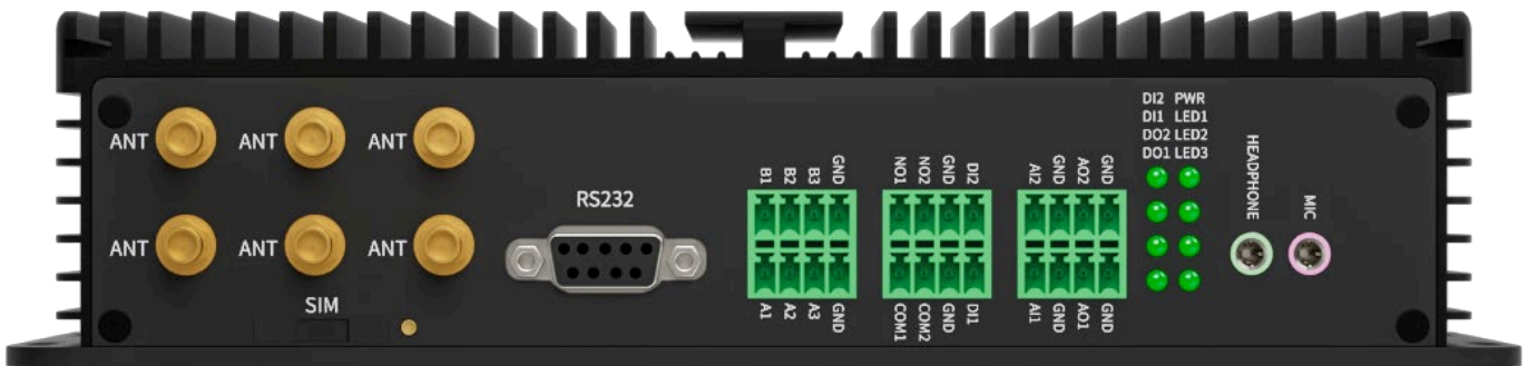
EG8200Pro Interface Identification-2
