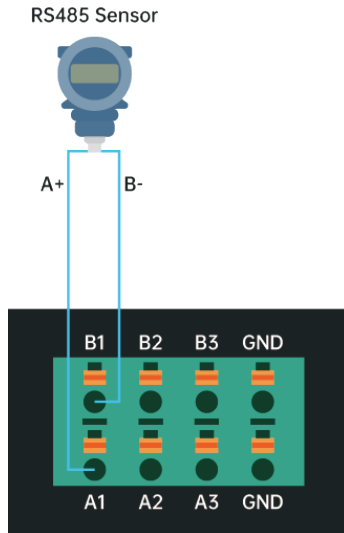
RS485 Wiring Diagram
