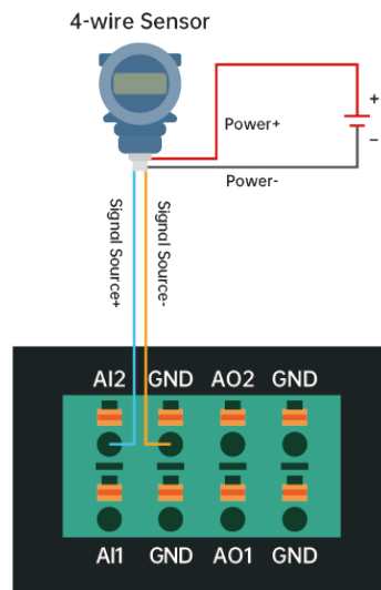
AI (4-wire) Wiring Diagram
