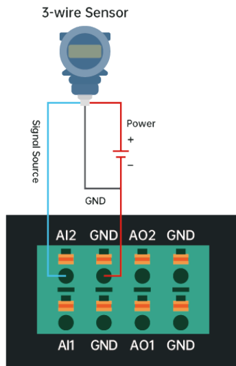
AI (3-wire) Wiring Diagram
