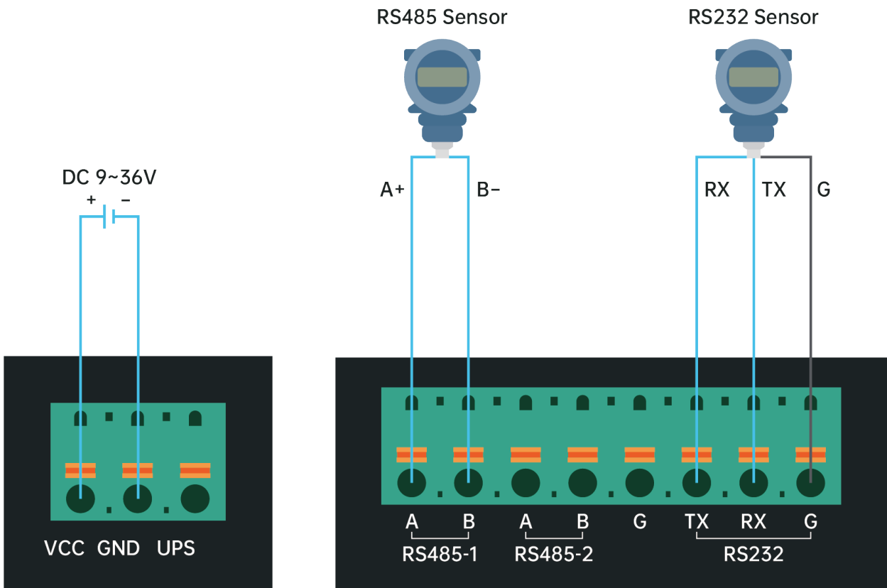
Power Wiring Diagram
